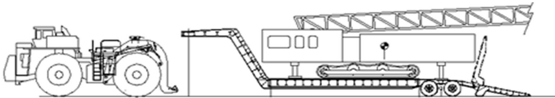
Rear Loading Design with Dual Rear Axle and Towing Attachment
